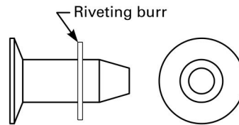
Belt Rivet
