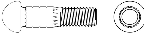
Bound-Body-Type High-Strength Bolt
