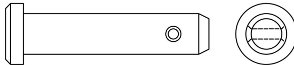
Clevis Pin
