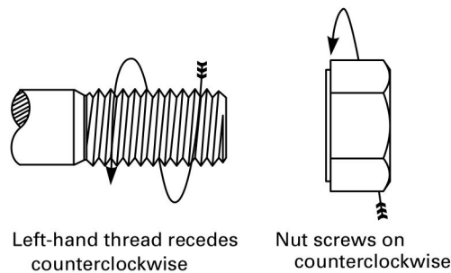
Left-Hand Thread
