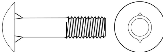
Round Head Fin Neck Bolt
