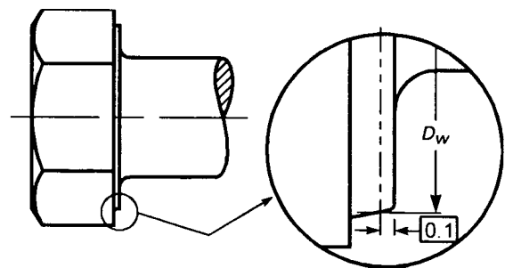
FIG. 1 WASHER FACE DETAIL
