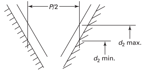
Fig. 46 Pitch Diameter, External Thread
