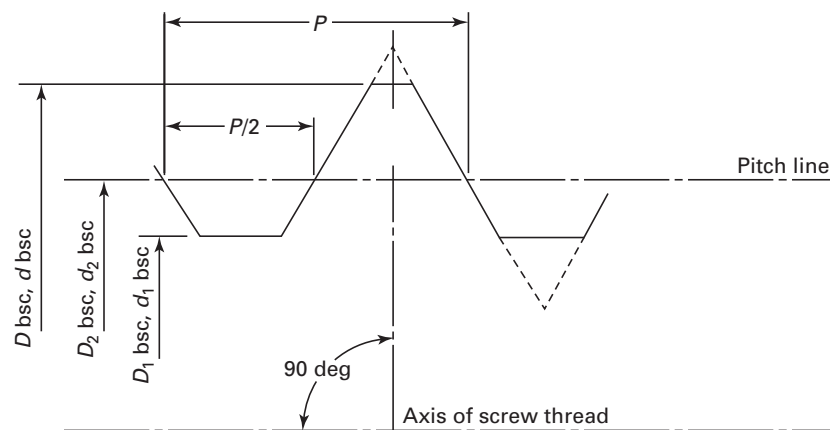
Fig. 49 Profile, Basic Thread
