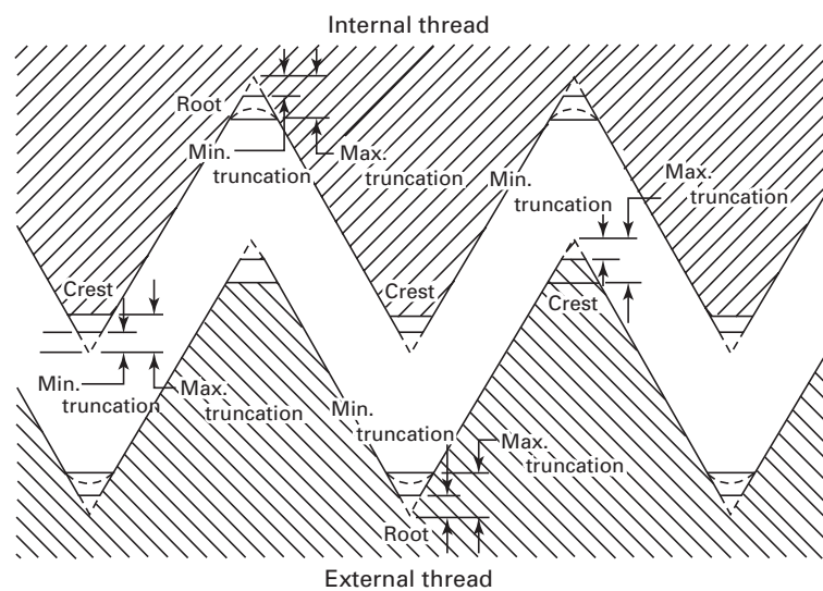
Fig. 57 Truncation
