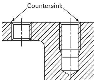
Fig. 7 Countersink
