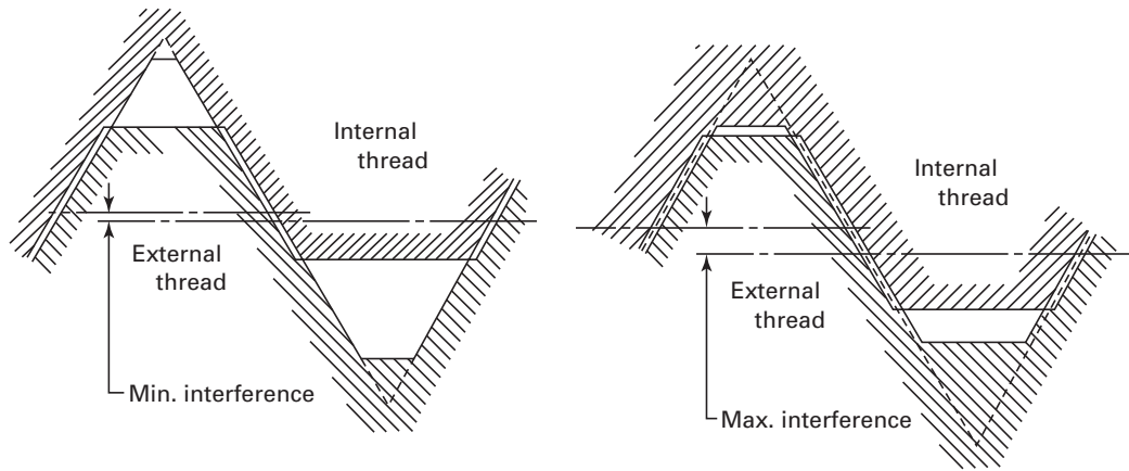
Fig. 24 Interference Fit
