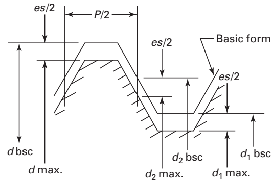
Allowance (Fundamental Deviation), External Thread
