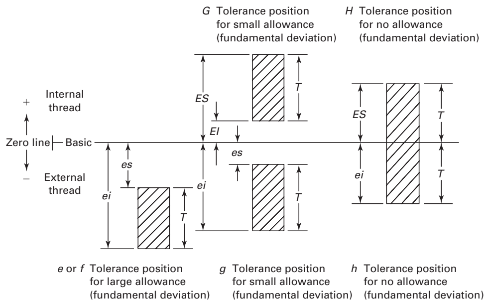
Fig. B-1 Metric Tolerance System for Screw Threads
