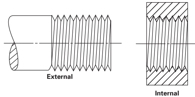
Fig. 54 Straight Thread
