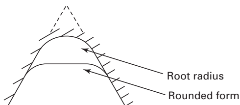
Internal Thread
