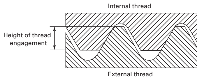
Fig. 20 Height of Thread Engagement
