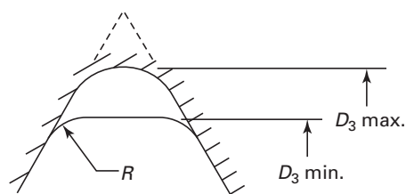
Fig. 35 Major Diameter, Internal Thread (Rounded Form)
