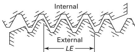
Fig. 30 Length of Thread Engagement
