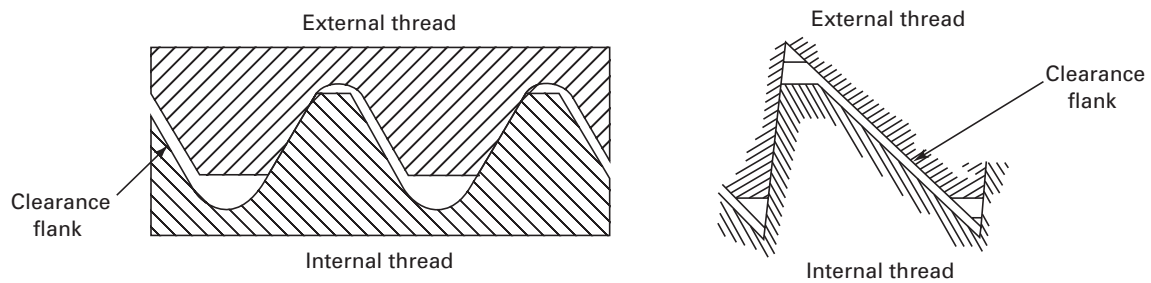
Fig. 6 Clearance Flank
