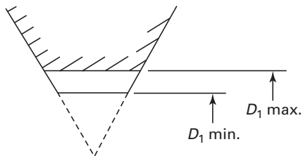
Fig. 40 Minor Diameter, Internal Thread
