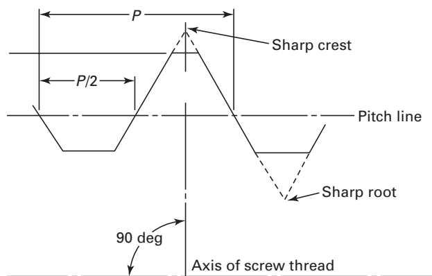
Fig. 52 Sharp Crest and Root
