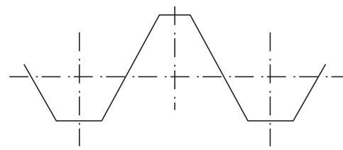
Fig. 15 Flat Form
