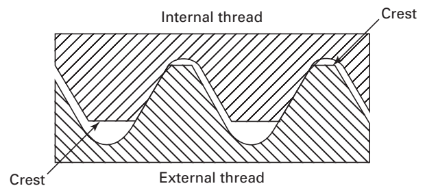
Fig. 8 Crest
