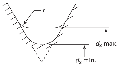
Fig. 39 Minor Diameter, External Thread (Rounded Form)
