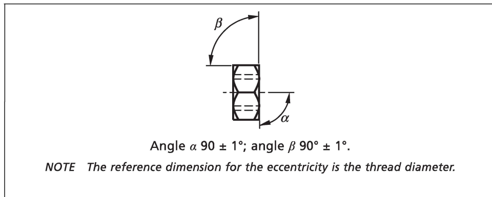
Figure E.17 Angularity of the nuts
