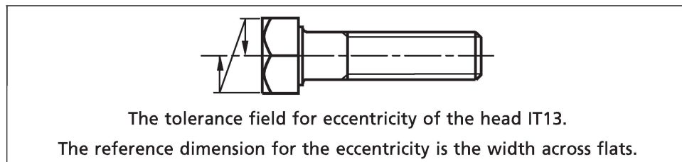
Figure E.8 Angularity of the head
