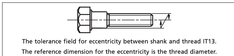
Figure E.9 Eccentricity between shank and thread
