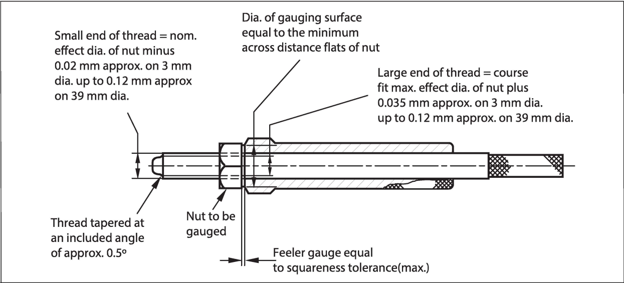
Figure B.1 Nut squareness gauge
