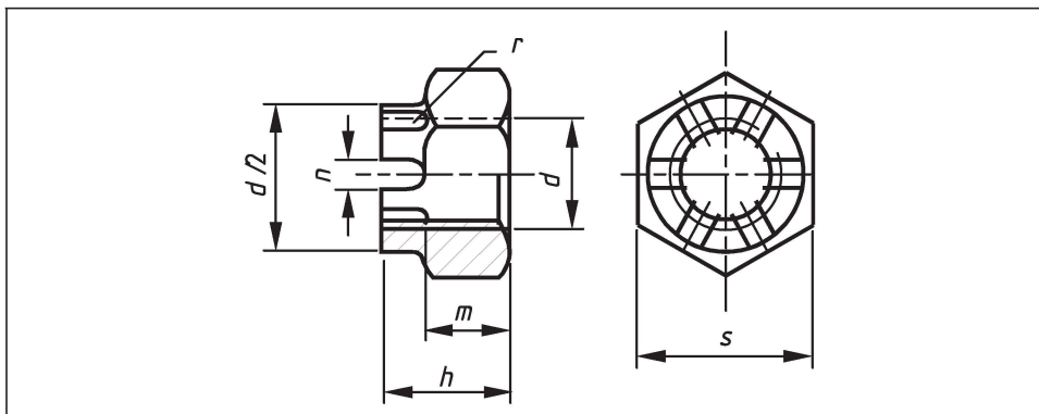
Figure 10 Castle nut. Sizes M12 to M39 only (six slots)
