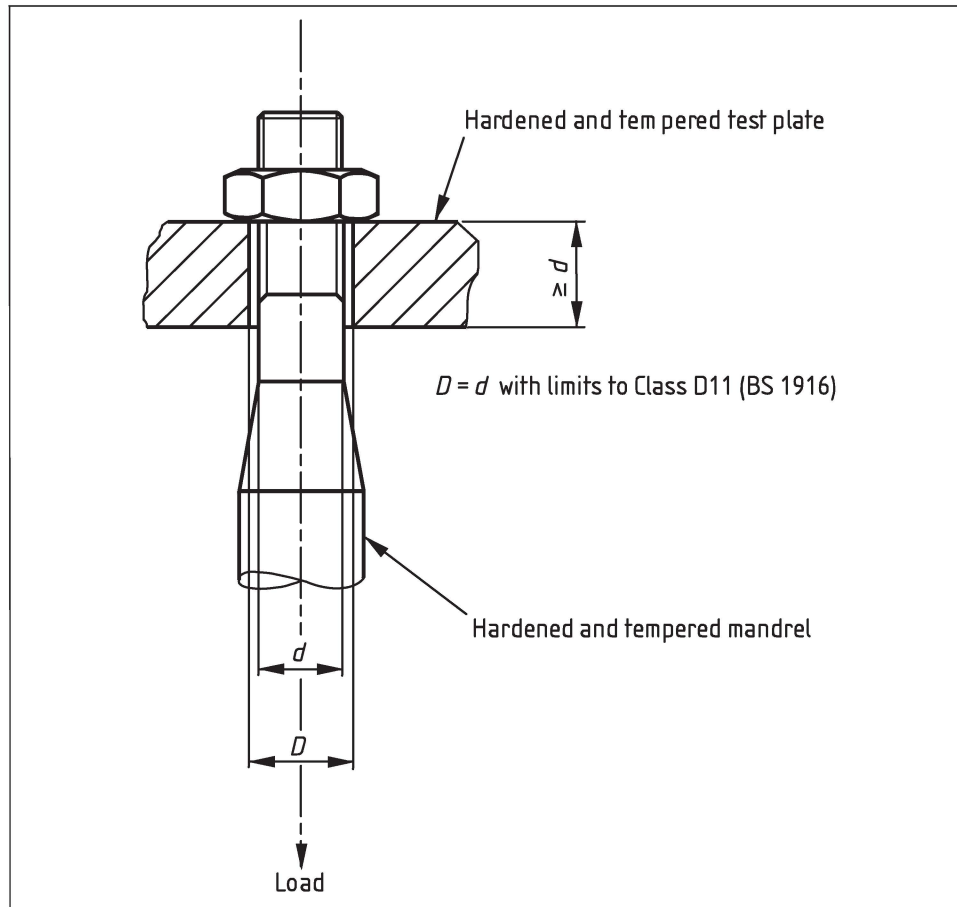
Figure C.1 Proof load test for nut
