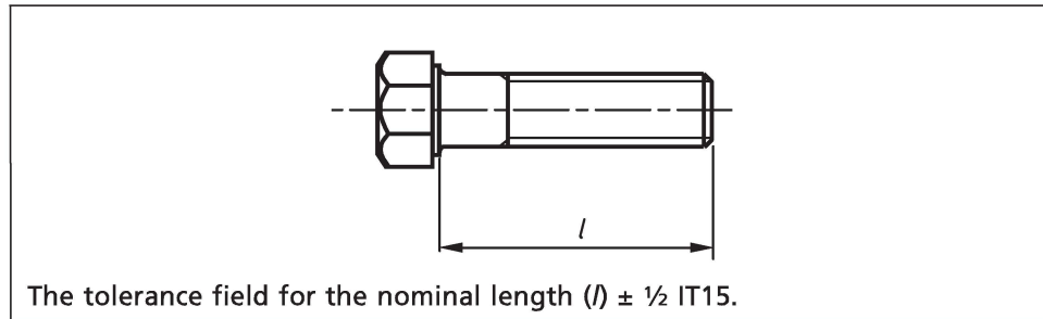
Figure E.6 Thread lengths
