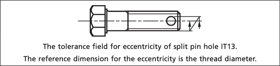
Figure E.10 Eccentricity of split pin hole
