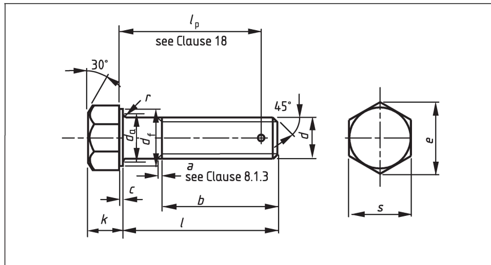
Figure 3 Hexagon head bolt, washer-faced
