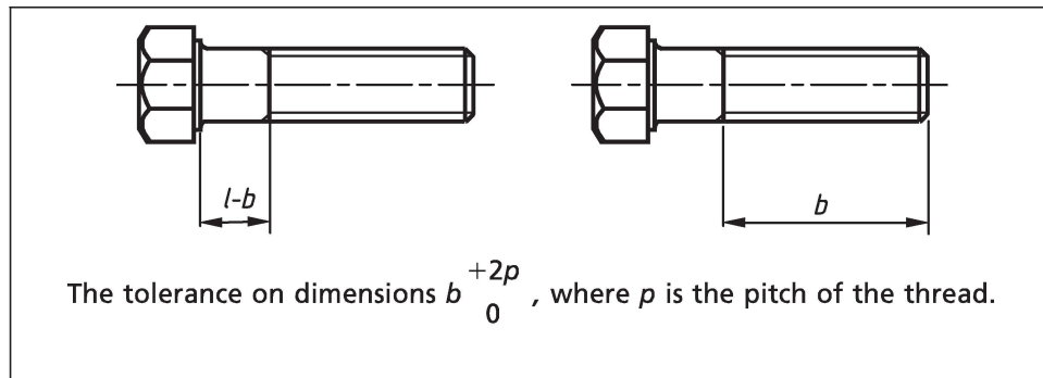
Figure E.7 Eccentricity of the head
