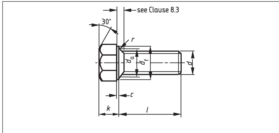
Figure 5 Full bearing head
