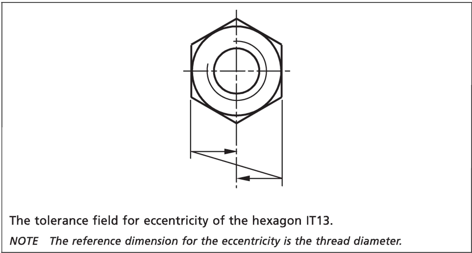
Figure E.15 Eccentricity of the hexagon
