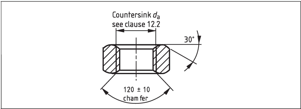
Figure 8 Enlarged view of nut countersunk
