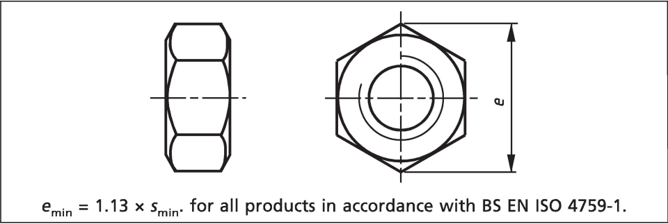
Figure E.12 Widths across corners
