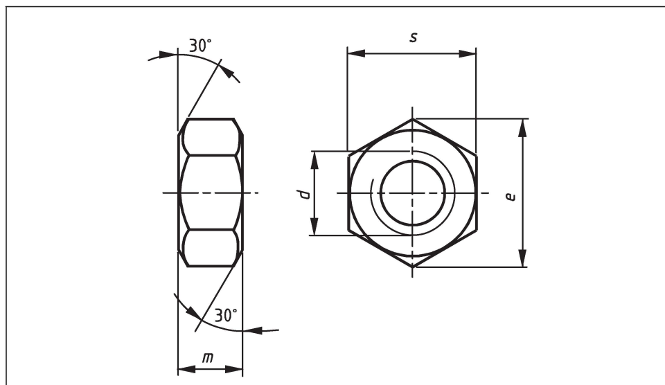
Figure 6 Normal thickness nut
