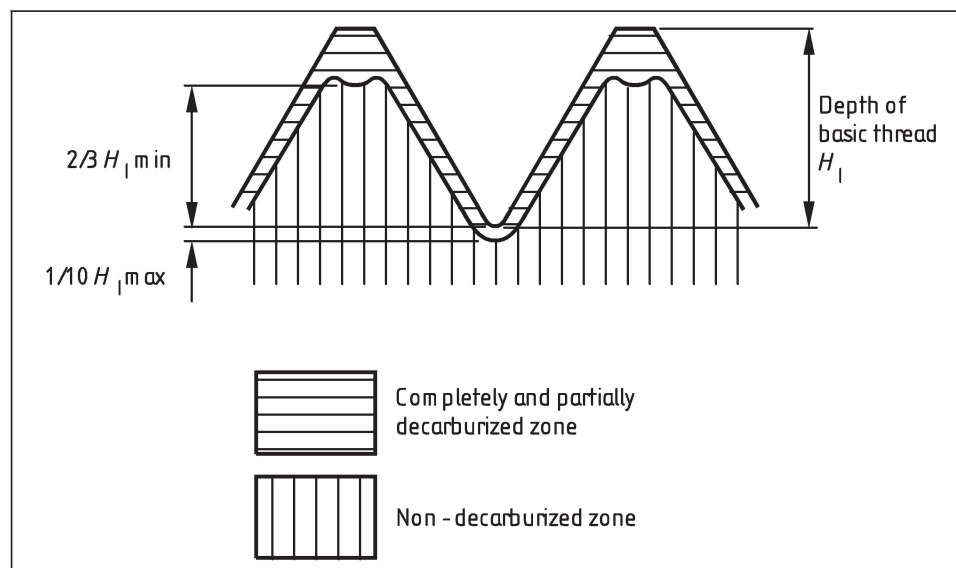
Figure 12 Depth of decarburization on steel bolts and screws
