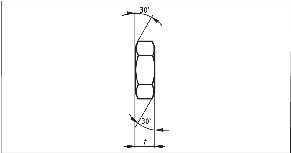
Figure 8 Enlarged view of nut countersunk
