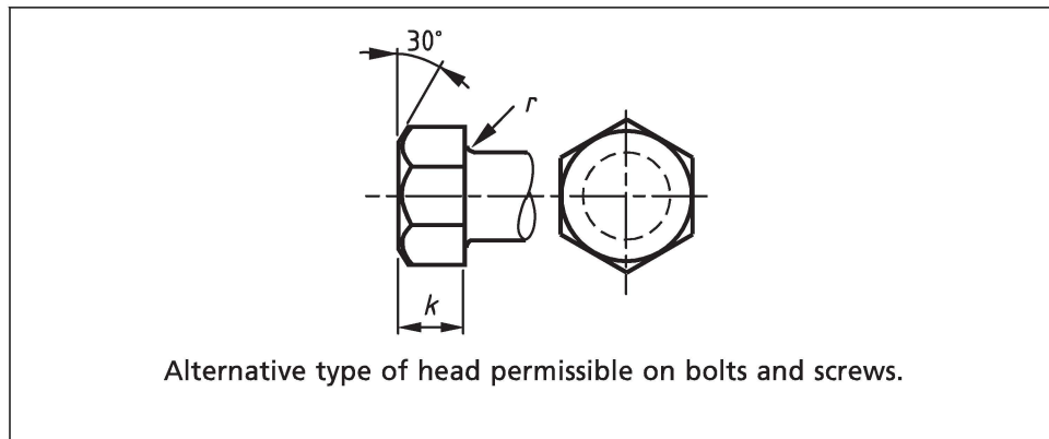
Figure 5 Full bearing head
