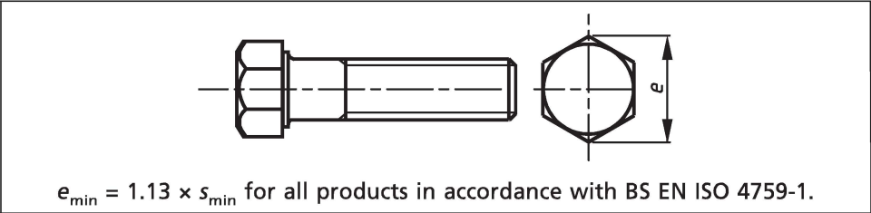
Figure E.3 Heights of heads
