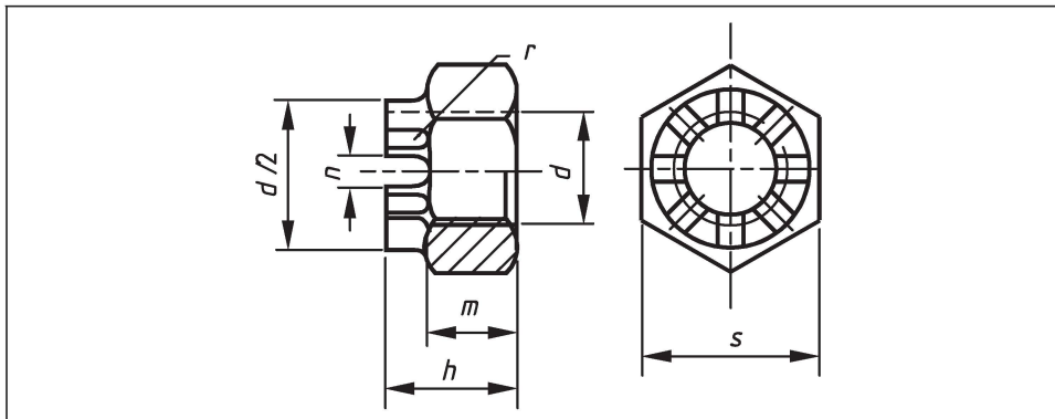
Figure 11 Castle nut. Sizes M42 to M68 only (eight slots)
