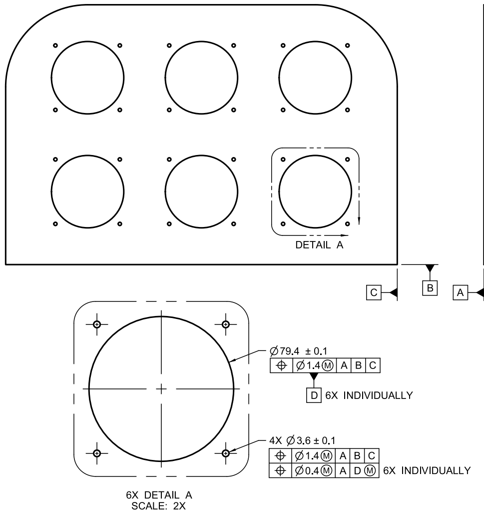
Figure 10-38 Multiple Patterns of Features
