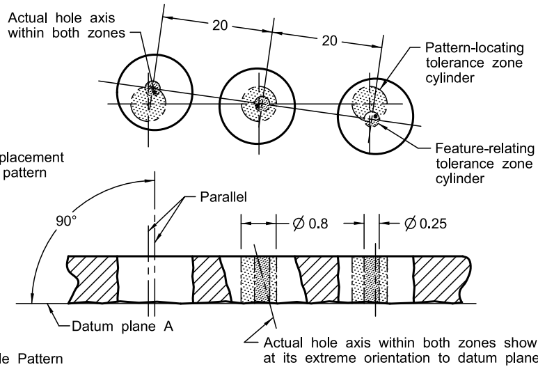
Figure 10-39 Hole Patterns Located by Composite Positional Tolerancing (Cont'd)
