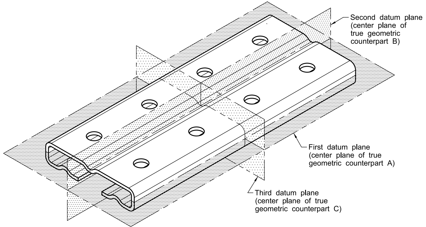
Figure 7-40 Irregular and Regular Features of Size as Datum Features (Cont'd)
