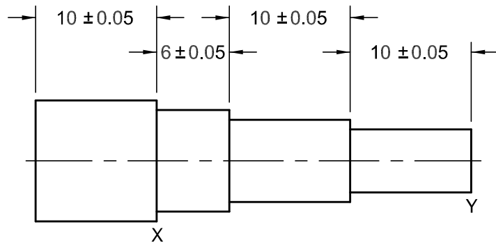
Figure I-1 Tolerance Accumulation
