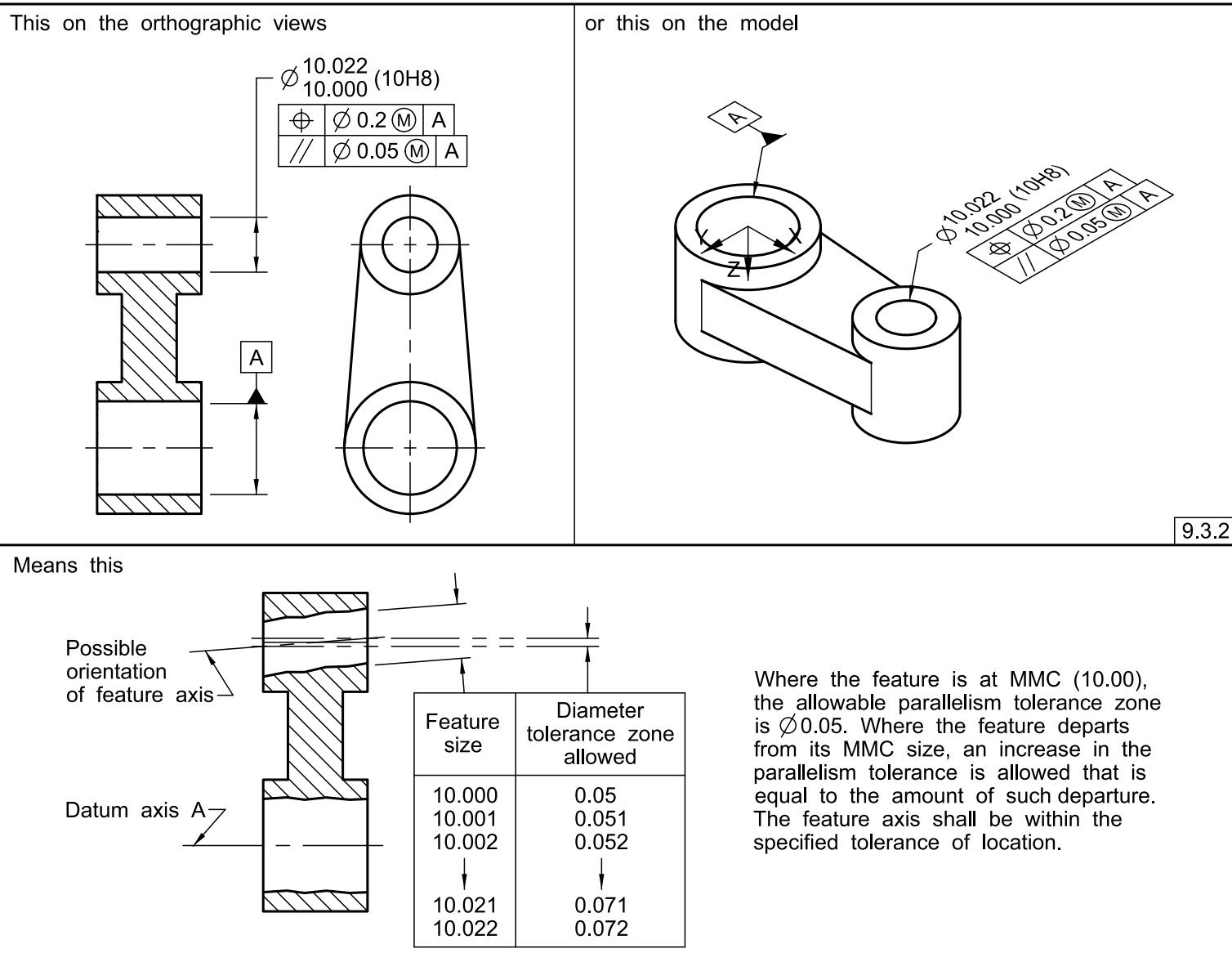
Figure 9-10 Specifying Parallelism for an Axis (Feature at MMC and Datum Feature RFS)
