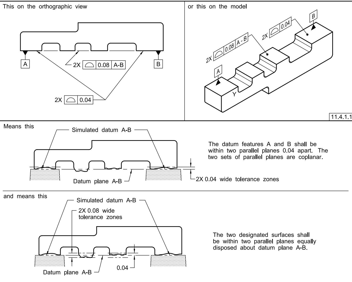
Figure 11-17 Specifying the Profile of a Surface for Coplanar Surfaces to a Datum Established by Two Surfaces
