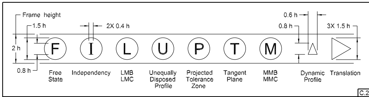
Figure C-4 Form and Proportion of Modifying Symbols
