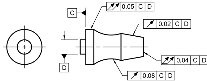
Figure 12-10 Specifying Runout to a Surface and Diameter
