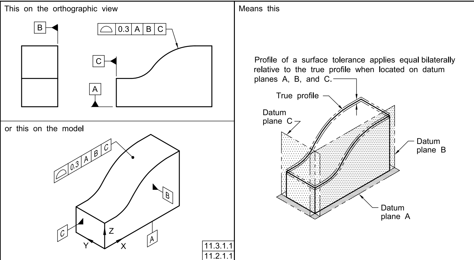
Figure 11-1 Profile of a Surface Application (Bilateral)
