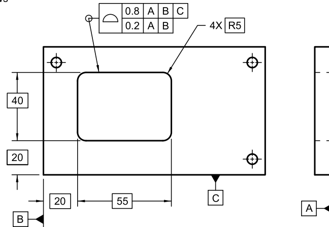
Figure 11-25 Composite Profile Tolerancing of a Feature
