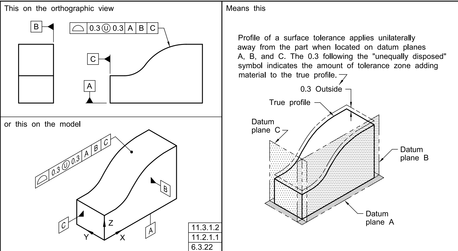
Figure 11-3 Profile of a Surface Application (Unilaterally Outside)
