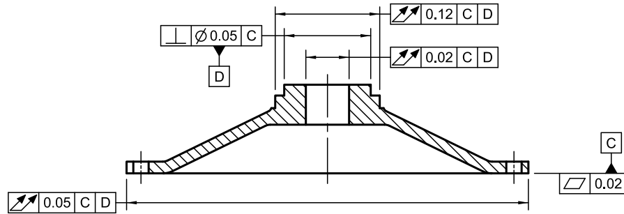
Figure 12-12 Specifying Runout Relative to a Surface and Diameter With Form Control Specified
