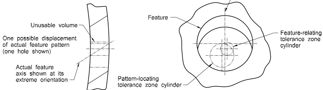
(b) Tolerance Zones for Radial Hole Pattern
