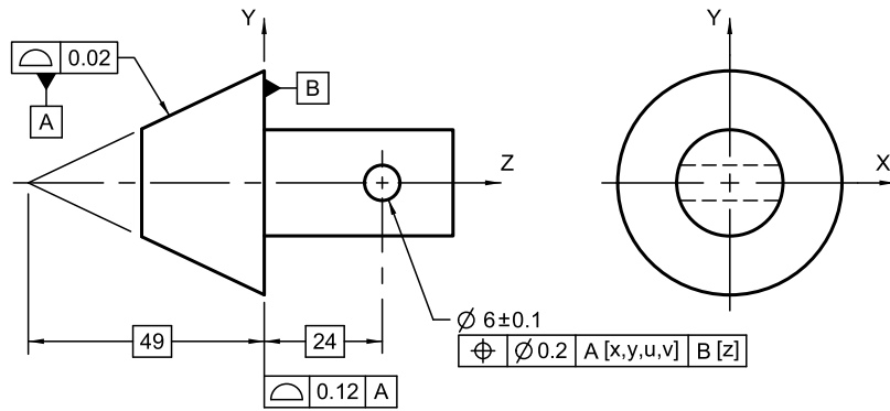
Figure 7-56 Conical Datum Feature Reference Customized to Constrain Four Degrees of Freedom
