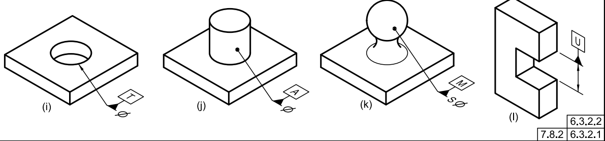
Figure 6-5 Placement of Datum Feature Symbol in Conjunction With a Feature Control Frame
