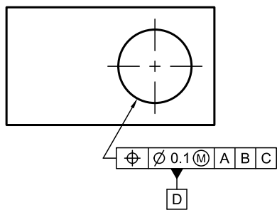
Figure 6-5 Placement of Datum Feature Symbol in Conjunction With a Feature Control Frame
