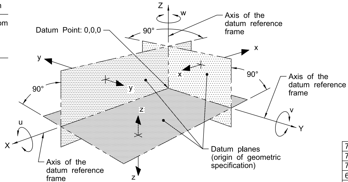
Figure 7-1 Datum Reference Frame
