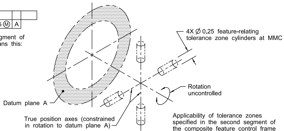
(b) Tolerance Zones for Radial Hole Pattern: FRTZF
