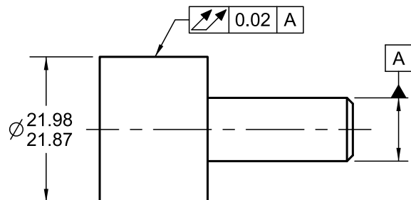
Figure 12-8 Specifying Total Runout Using a Large Size Tolerance and a Small Runout Tolerance
