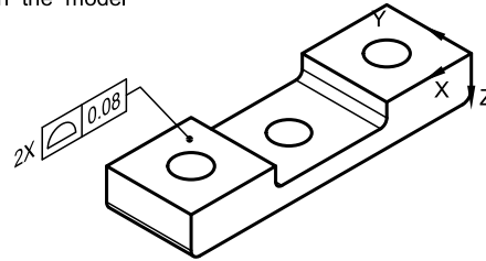
Figure 11-16 Specifying the Profile of a Surface for Coplanar Surfaces
