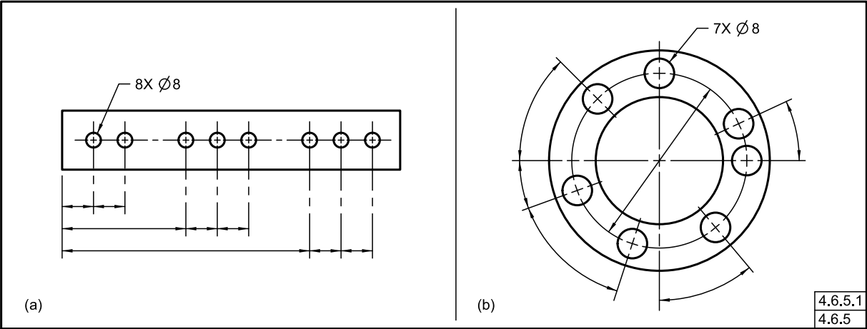
Figure 4-51 Repetitive Features
