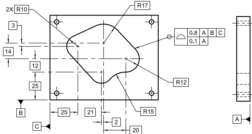
Figure 11-24 Composite Profile Tolerancing of an Irregular Feature
