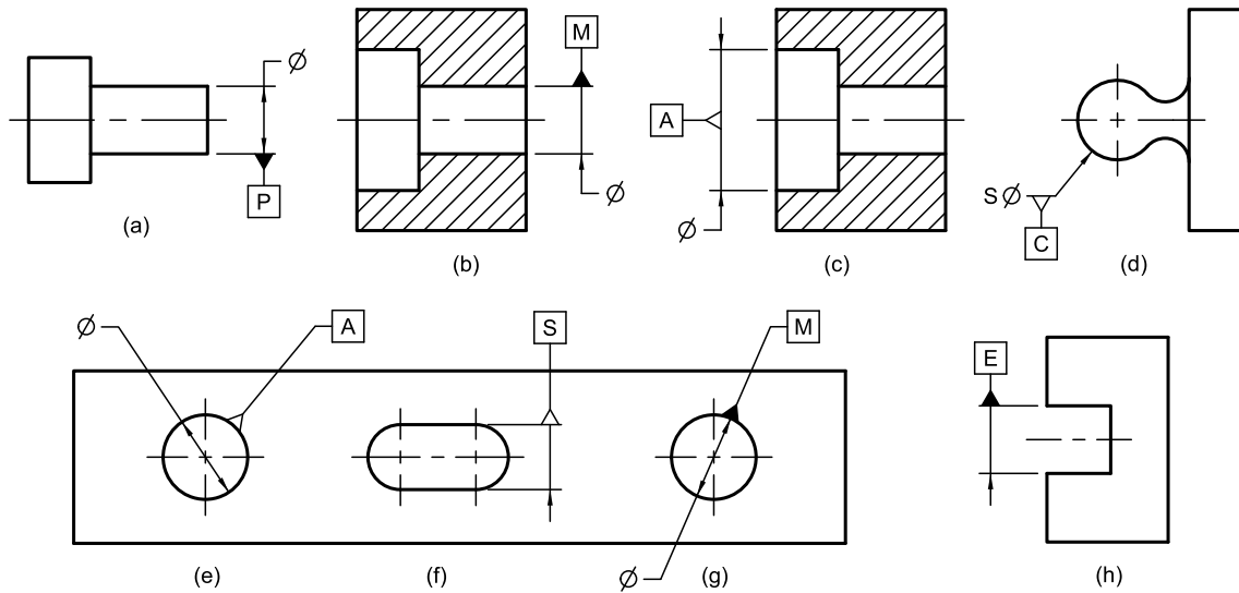
Figure 6-4 Placement of Datum Feature Symbols on Features of Size
