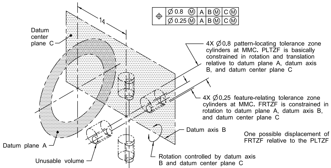
(a) Tolerance Zones for Radial Hole Pattern
