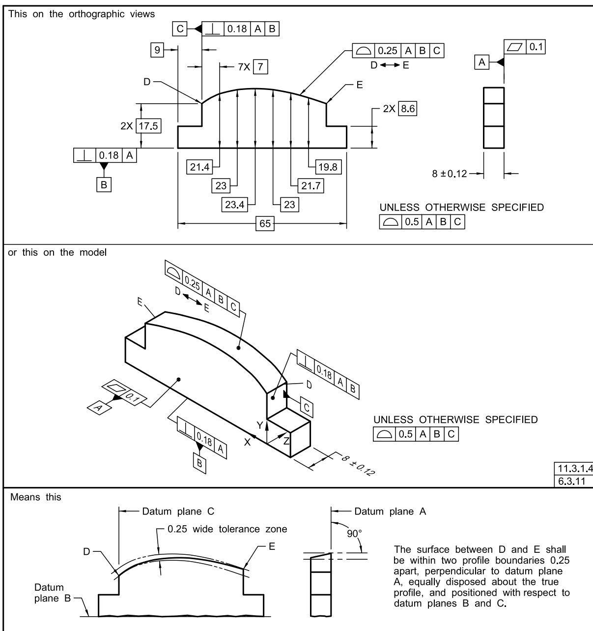
Figure 11-9 Specifying Profile of a Surface Between Points
