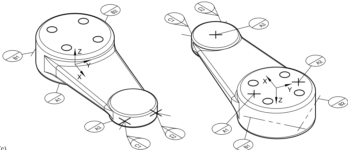
Figure 7-58 Application of Movable Datum Targets (Cont'd)
