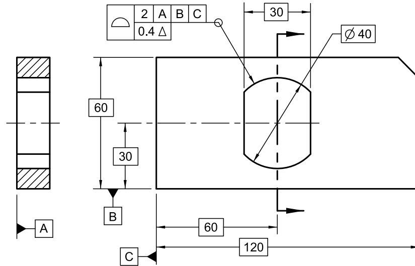
Figure 11-35 Composite Profile With Dynamic Profile to Control Form
