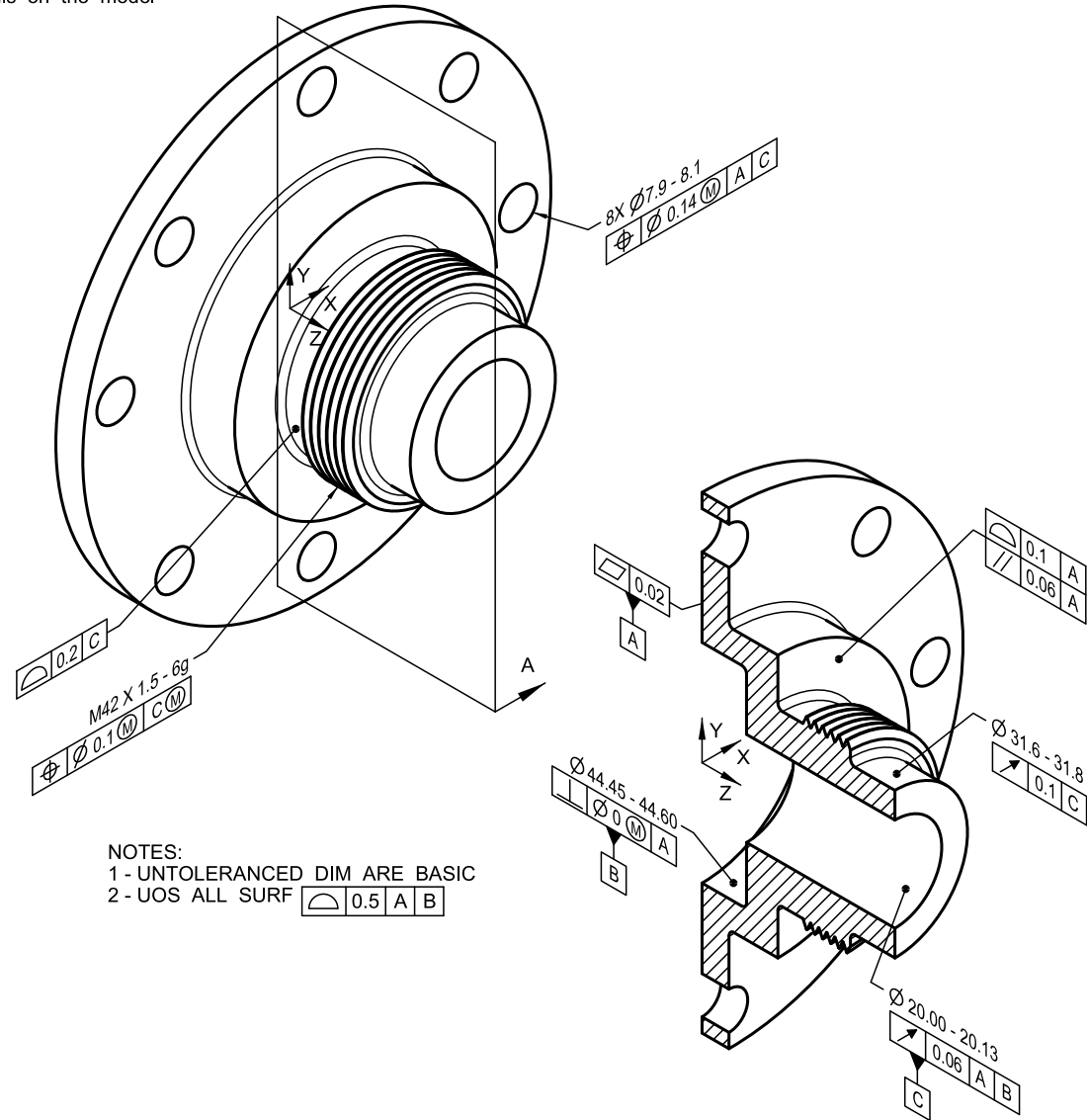
Figure 6-30 Feature Control Frame Placement (Cont'd)
