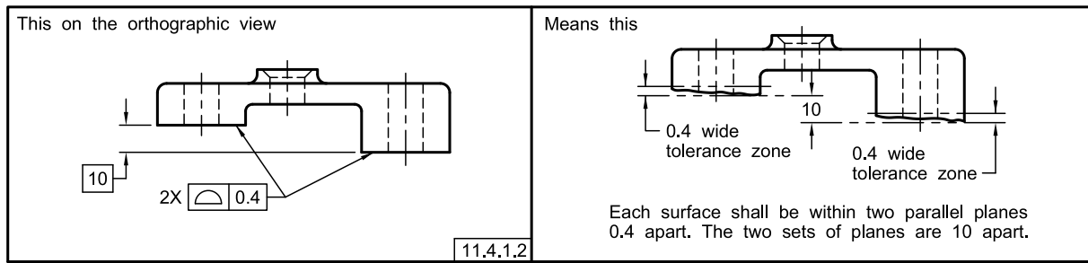
Figure 11-18 Specifying the Profile of a Surface for Stepped Surfaces
