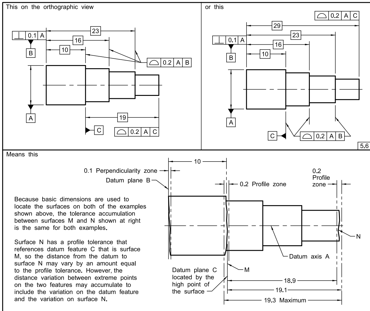
Figure 5-5 Tolerance Accumulation: Multiple Datum Reference Frames
