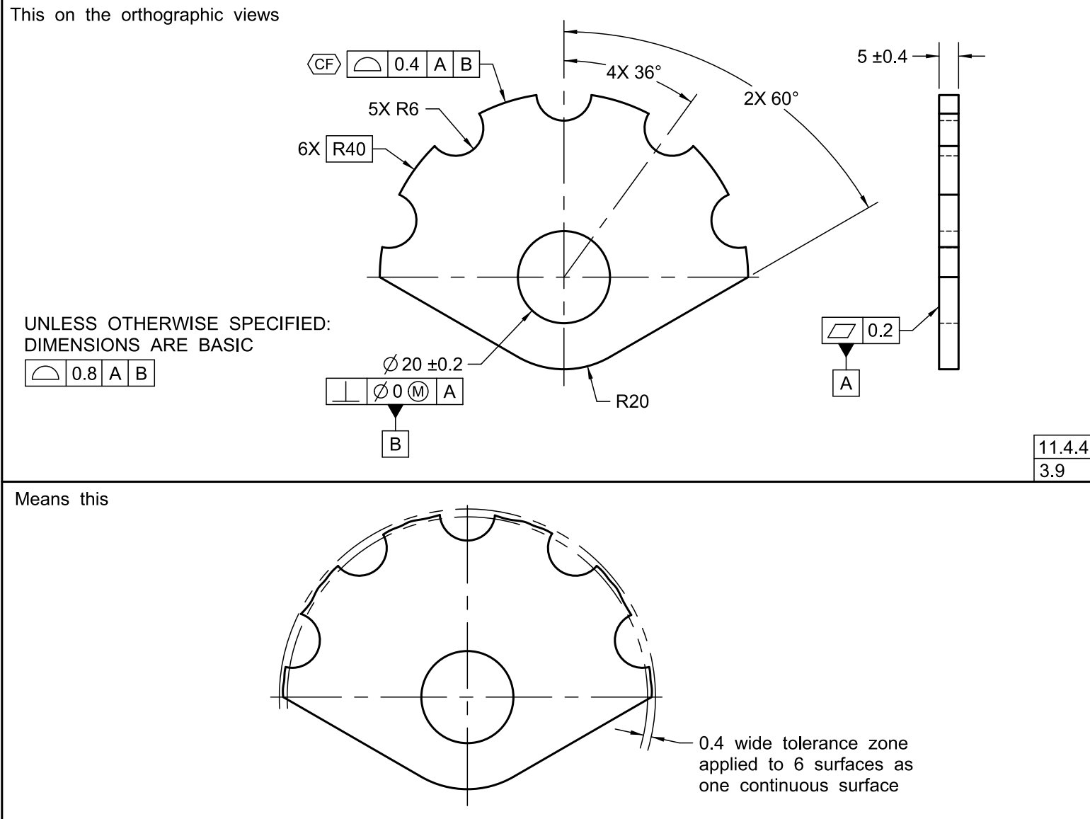
Figure 11-23 “Continuous Feature” Symbol Application in a Profile Tolerance
