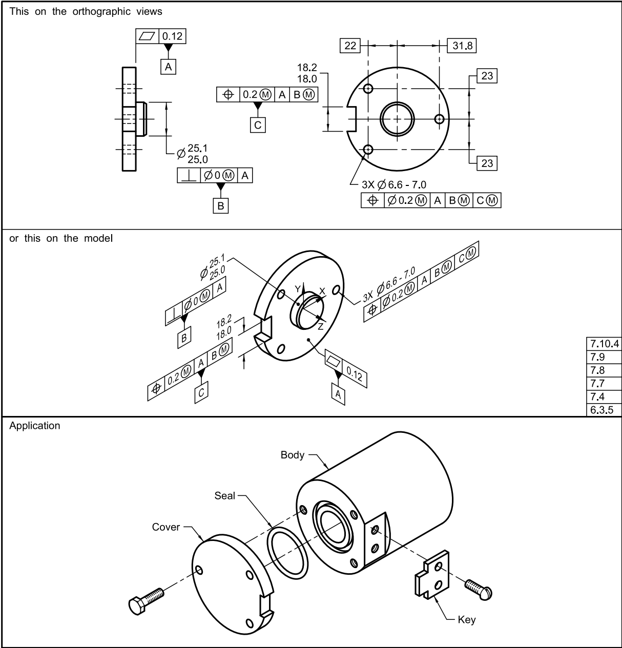
Figure 7-4 Part Where Rotational Constraint Is Important
