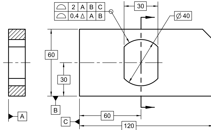
Figure 11-37 Use of Dynamic Profile in a Two-Single-Segment Profile Tolerance
