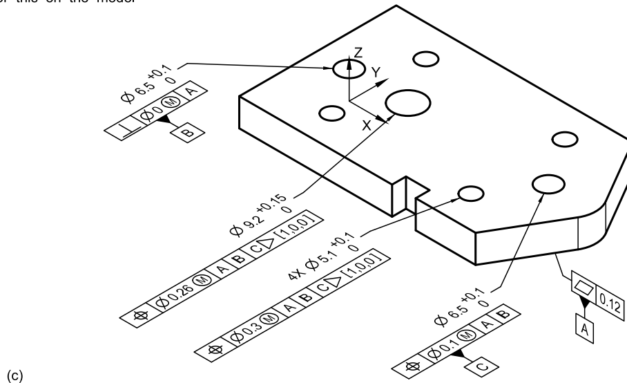
Figure 7-12 Development of a Datum Reference Frame With Translation Modifier (Cont'd)
