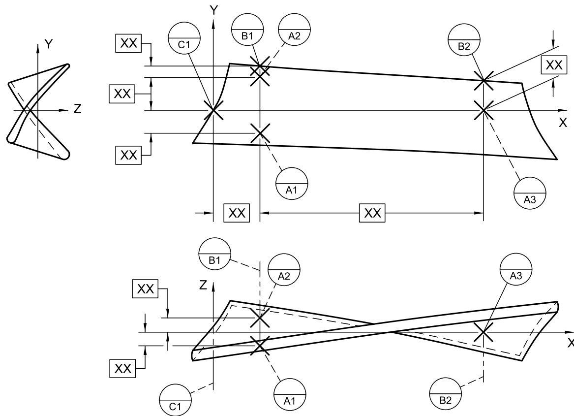
Figure 7-53 Datum Targets Used to Establish Datum Reference Frame for Complex Part
