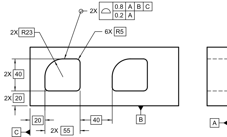
Figure 11-26 Pattern Located by Composite Profile Tolerancing — Repeated Primary Datum Feature Reference
