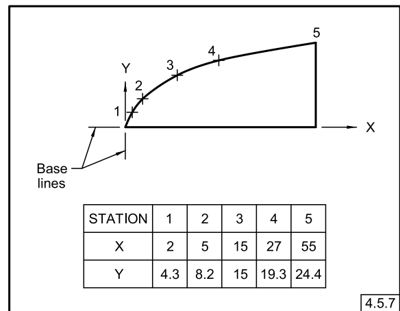
Figure 4-32 Tabulated Outline
