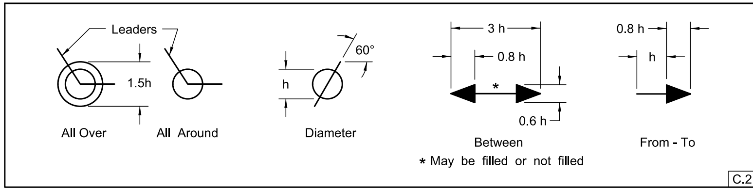
Figure C-3 Form and Proportion of Geometric Dimensioning Symbols
