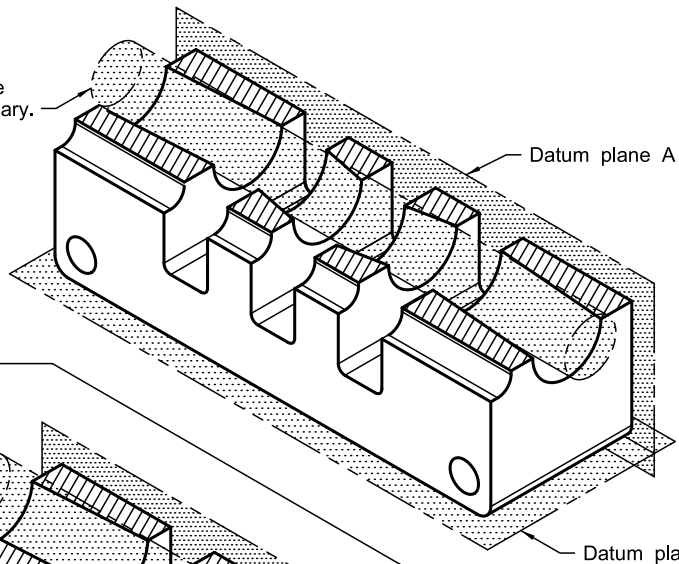
Figure 10-45 Positional Tolerancing for Coaxial Holes of Same Size, Partial (Parallelism) Refinement of Feature-Relating Axis Relative to Datums A and B With Further Refinement of Parallelism to Datum A (Cont'd)
