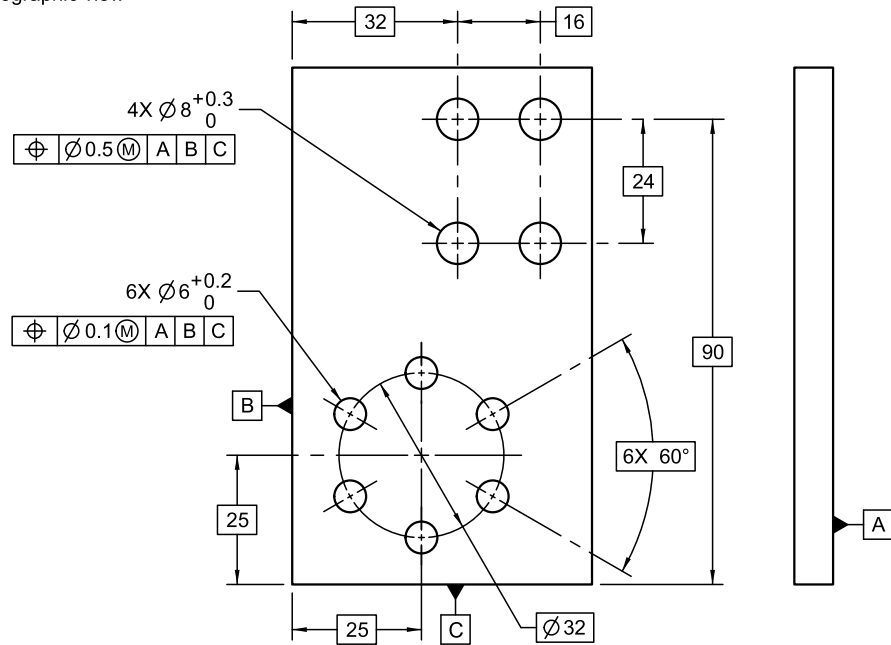
Figure 10-53 Multiple Patterns of Features, Simultaneous Requirement
