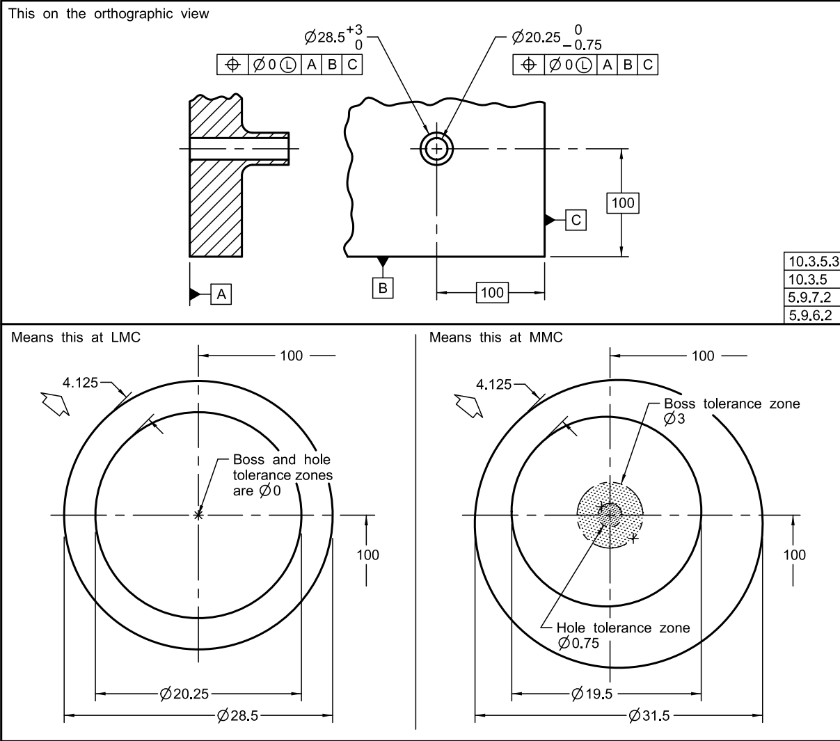
Figure 10-15 Zero Tolerance at LMC Applied to Boss and Hole
