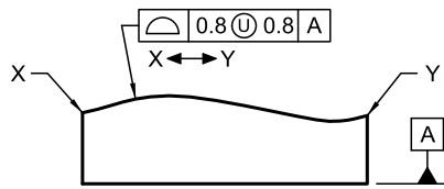
(c) Unilateral tolerance (outside)
