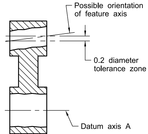
Figure 9-9 Specifying Parallelism for an Axis (Both Feature and Datum Feature RFS)
