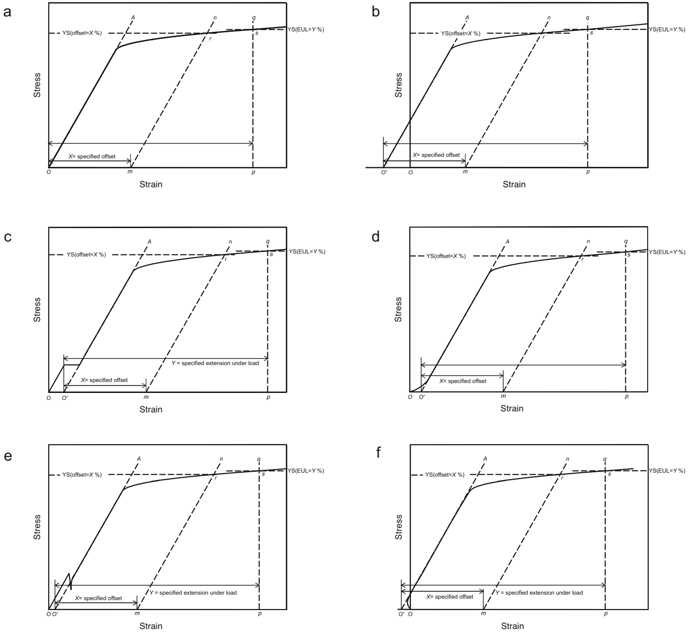
FIG. X5.1 Schematic Stress-strain Diagram
