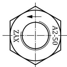
Figure 8 — Example of marking for left-hand thread
