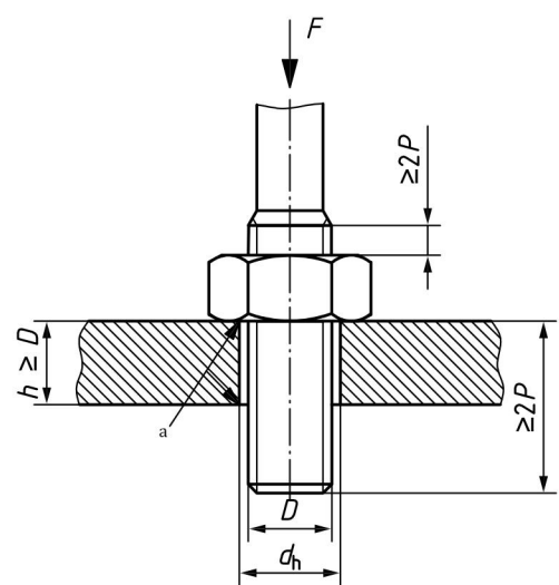
Figure 2 — Axial tensile test
