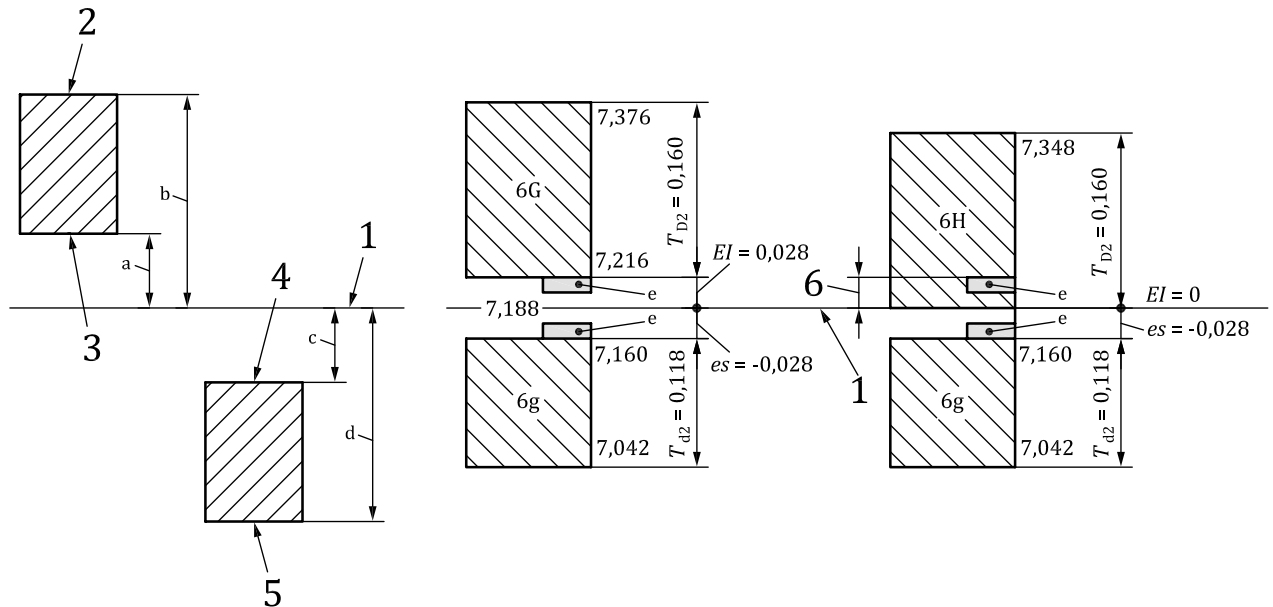
a) Internal/external thread
