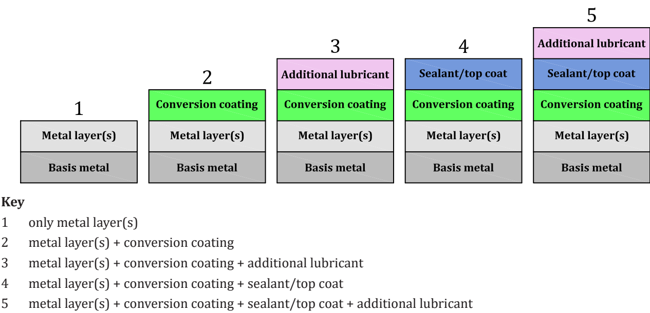
Figure 1 — Basic electroplated coating systems (schematic)
