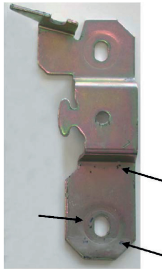
b) Same part after 408 h NSS testing
