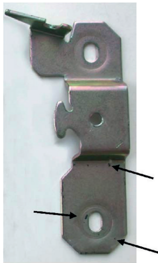
a) Part after 168 h NSS testing
