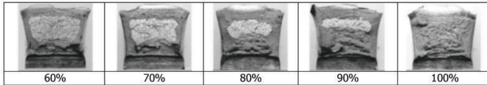
(a) Shear Fracture Appearance Charts
