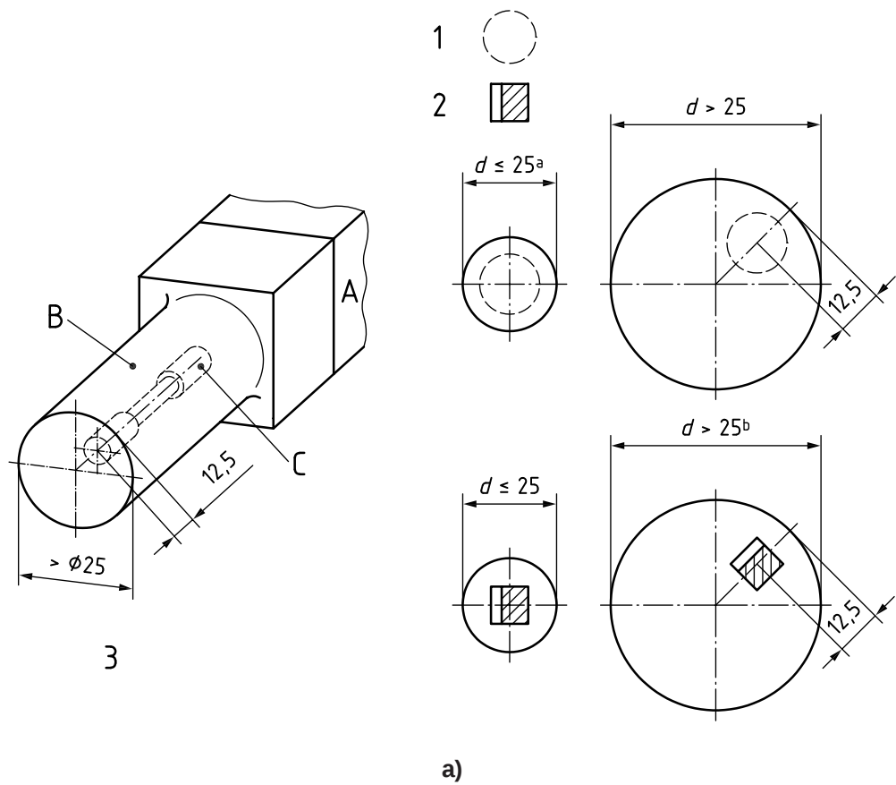
Figure 2 — Location of the test pieces in bars, seamless rolled rings and rods (continued)
