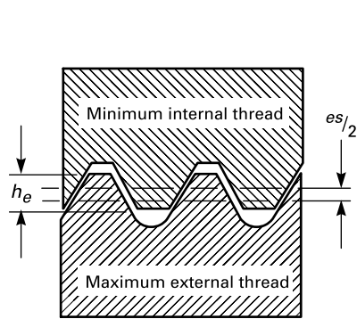
Thread With an Allowance
