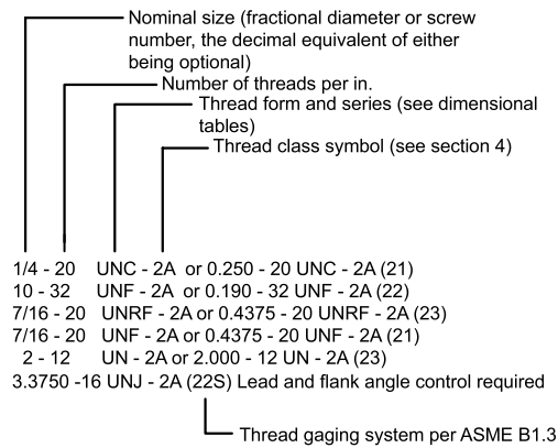
Figure 13 Basic Method of Designating Screw Threads
