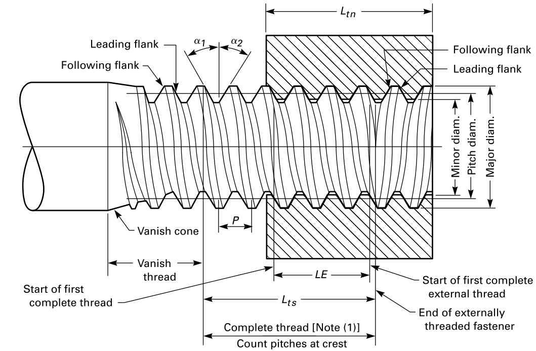
Figure 16 Application of General Thread Symbols
