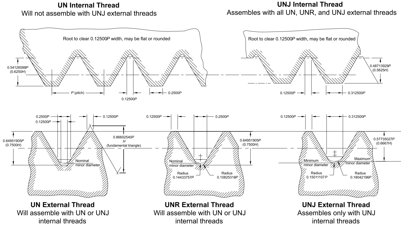
Figure A-1 Identification of 60-deg Inch Screw Threads Within the Scope of the ASME B1 Committee
