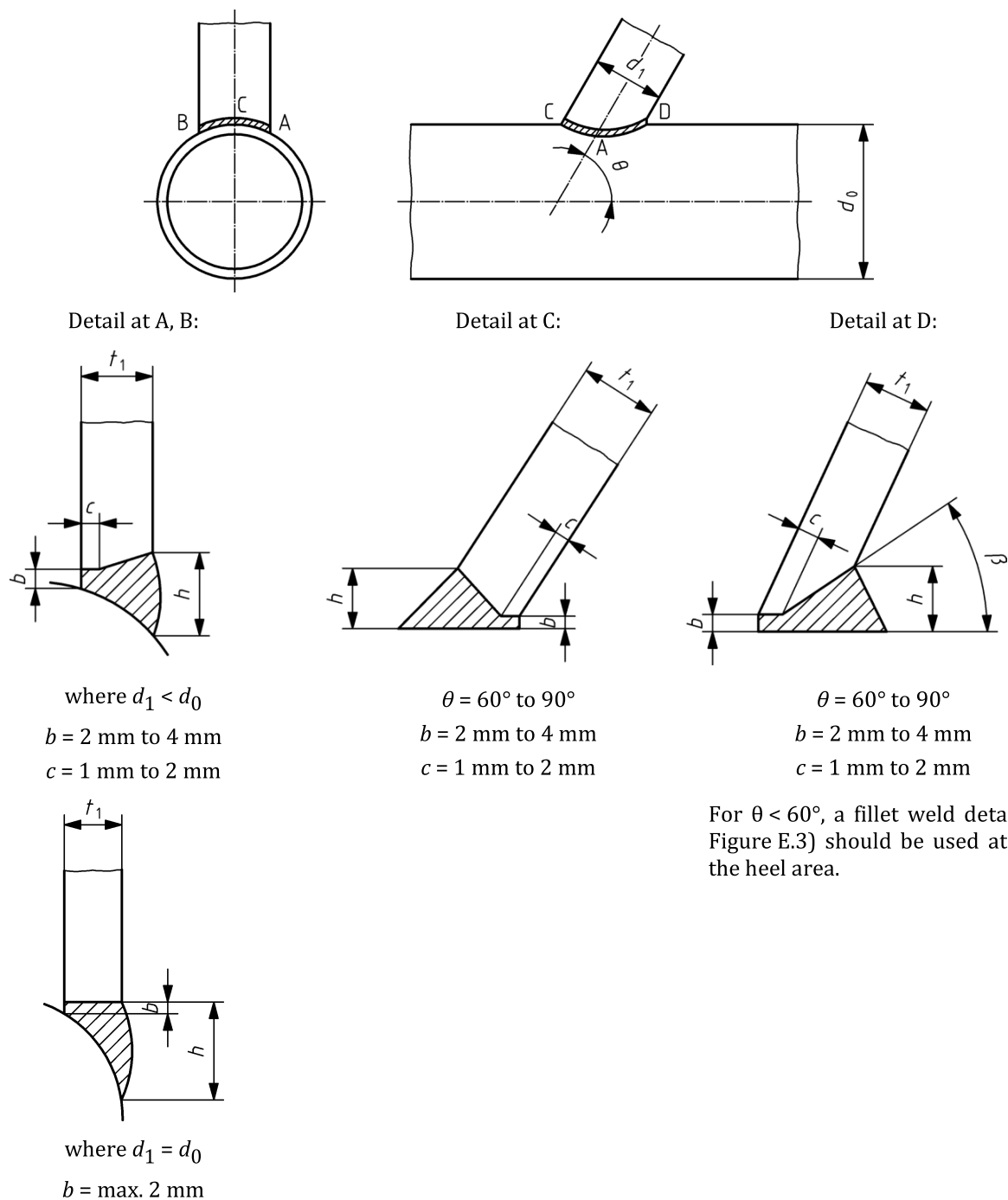
Figure E.2 — Weld preparation and fit-up - Butt welds in circular hollow sections brace to chord joints
