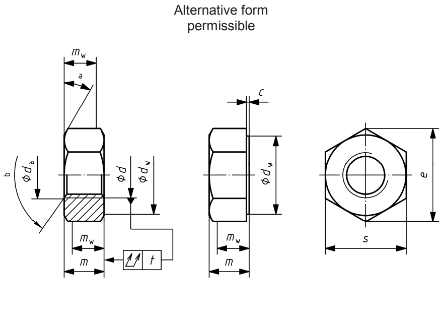
Figure 3 — Dimensions of nuts
